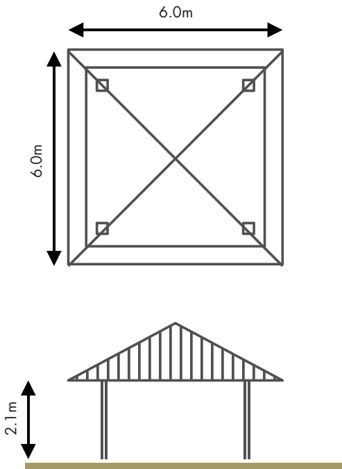
Recommended shelter dimension for 10 to 12 people
